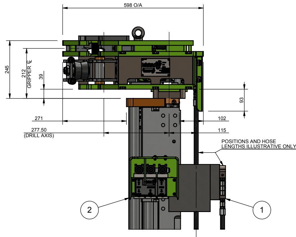
FRONT VIEW WITH LOBSTER SCALE 1:10
