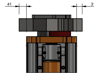
SIDE VIEW WITH TSRU SE HEADPLATE SCALE 1:10
