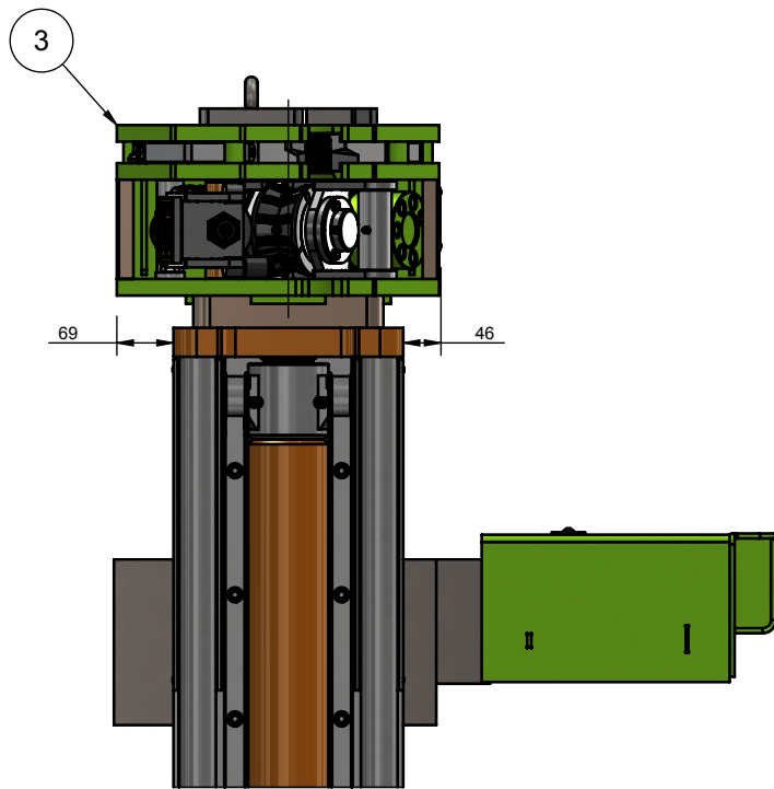
SIDE VIEW WITH LOBSTER SCALE 1:10
