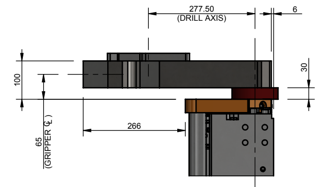
FRONT VIEW WITH TSRU SE HEADPLATE SCALE 1:10
